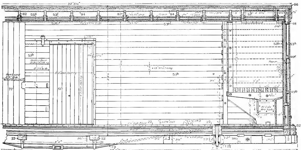
Fig. 279. Part Longitudinal Section.
